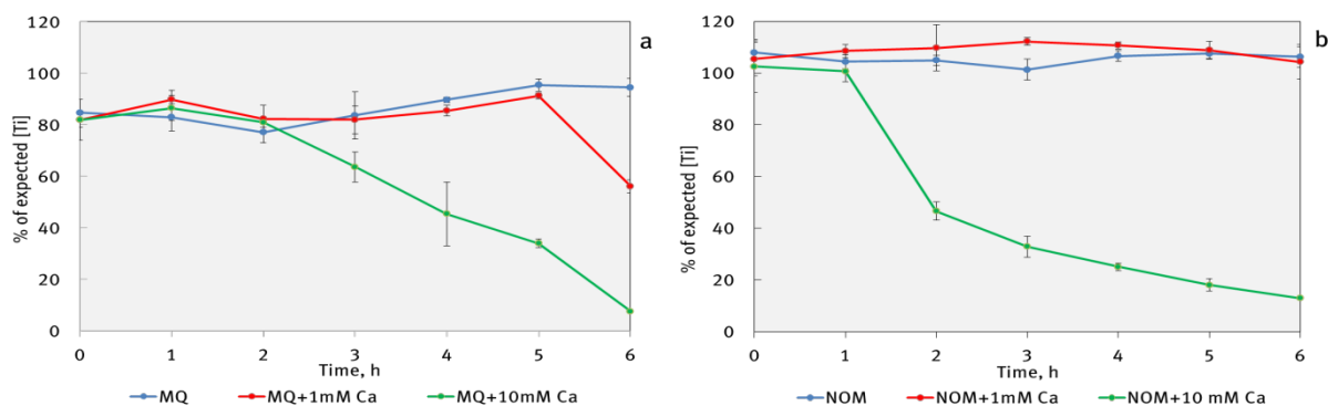
Figure 18: Agglomeration behavior of \text{TiO}_2 (NM105) nanoparticles. (a) in 0, 1, 10 mM \text{Ca}(\text{NO}_3)_2 media, (b) in 0, 1, 10 mM \text{Ca}(\text{NO}_3)_2 and 30 ppm DOC (SRNOM) media. Error bars from 3 replicate experiments.
