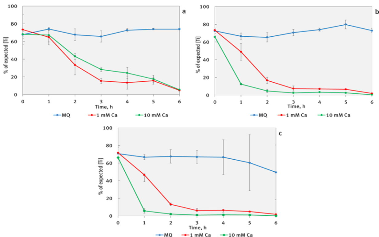
Figure 23: Agglomeration behavior of TiO 2 (NM105) nanoparticles at pH=8.5. pH values were established in presence of (a) 1 mM NaHCO 3 , (b) 5 mM NaHCO 3 , (c) 10 mM NaHCO 3 and the pH values remained stable during all experimental procedures.
