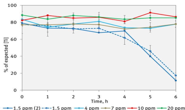
Figure 20: Agglomeration behavior of TiO 2 (NM105) nanoparticles in 1 mM Ca(NO 3 ) 2 and different concentrations of DOC (SRNOM). Error bars from 3 replicate experiments.
