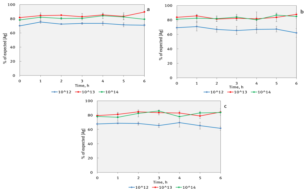
Figure 26: Dispersion stability of Ag (NM300K) particles in the dispersions of various density: 10 12 , 10 13 , 10 14 particles /L. (a) in MQ, (b) in 1 mM Ca(NO 3 ) 2 and (c) in 5 mM Ca(NO 3 ) 2 .
