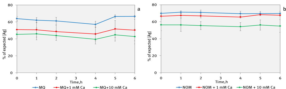
24: Agglomeration behavior of Ag (NM300K) nanoparticles in dispersion with established pH=8.5. (a) in 0, 1, 10 mM \text{Ca}(\text{NO}_3)_2 media, (b) in 0, 1, 10 mM \text{Ca}(\text{NO}_3)_2 and 30 ppm DOC (SRNOM) media.
