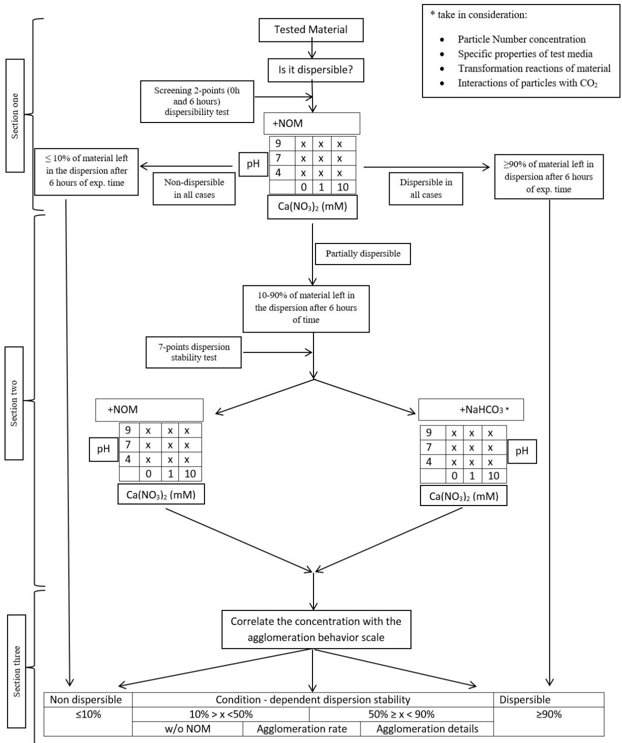
Figure 29: Suggested tiered agglomeration behavior scheme
