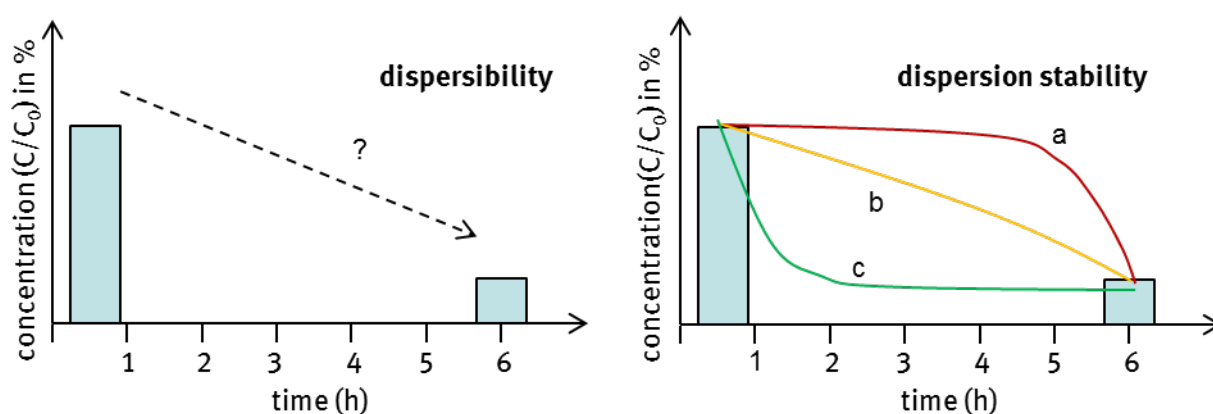
Figure 3: Possible types of particle agglomeration behavior in dispersibility test and in dispersion stability test.
